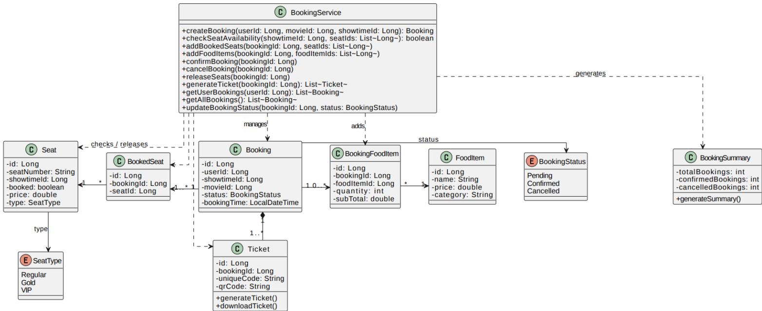
Class Diagram - Booking Service
