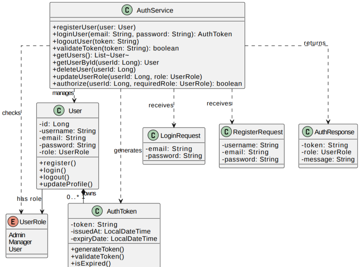
Class Diagram - Authentication / Authorization Service
