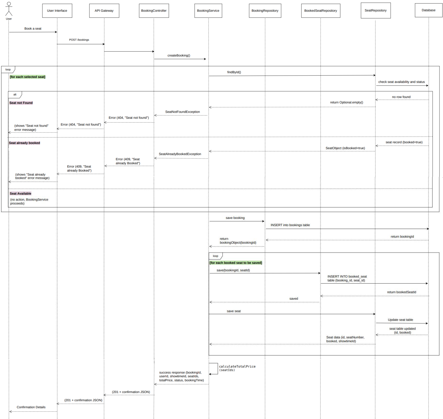
Seat Booking Sequence Diagram (User Use Case)
