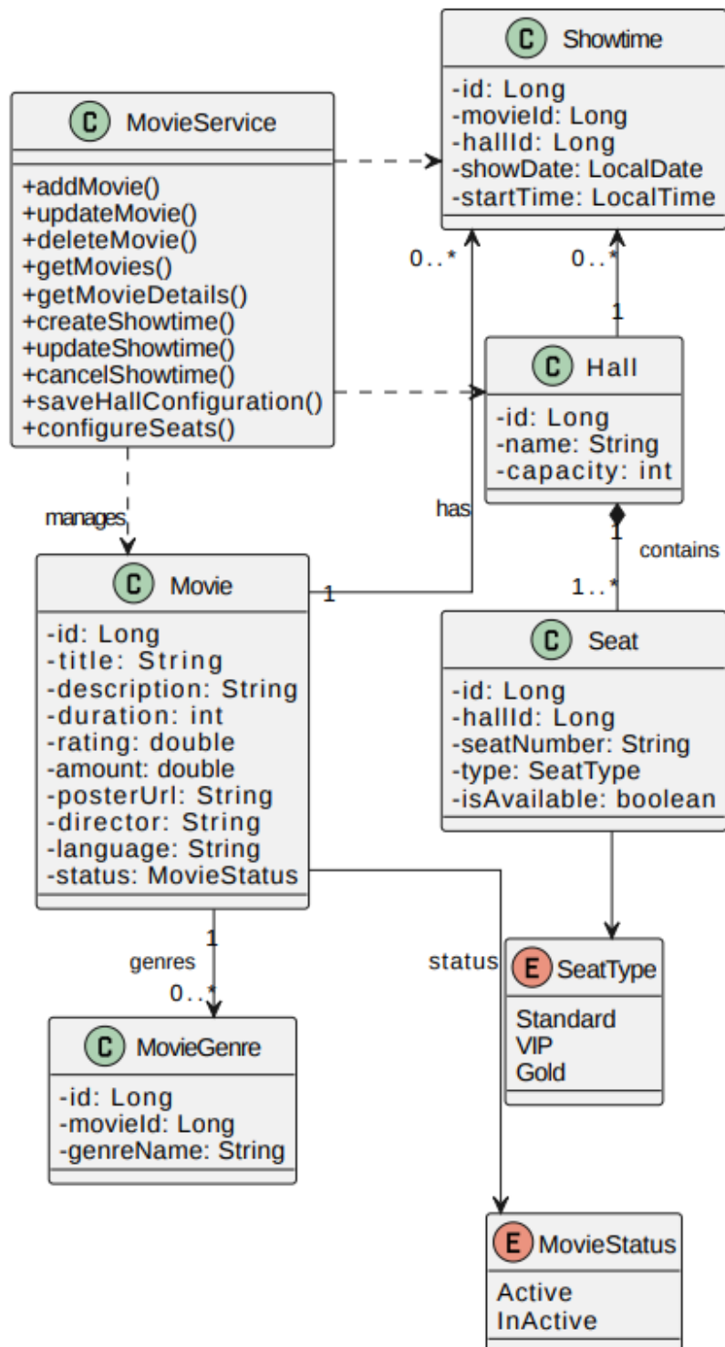
Class Diagram - Movie Service
